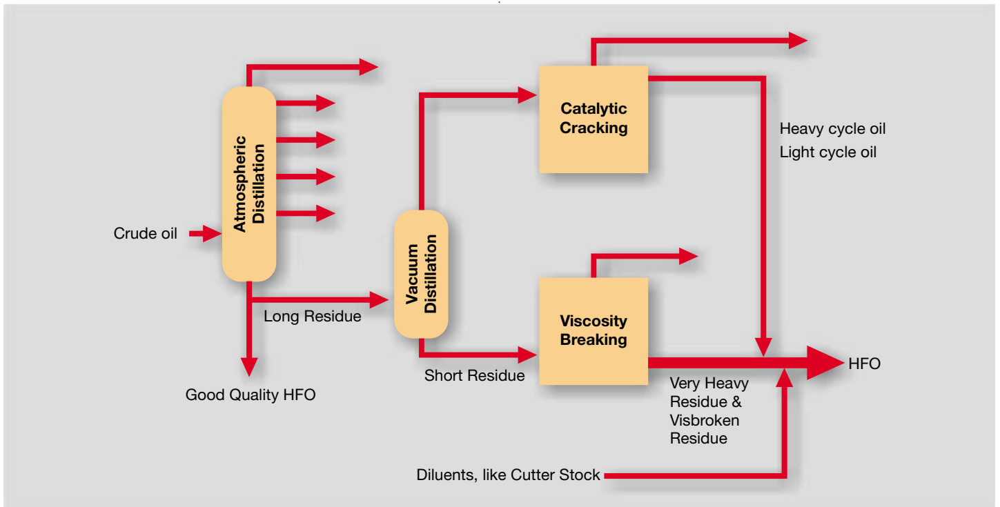
Fig. 2 Example of modern fuel refinery configuration.
